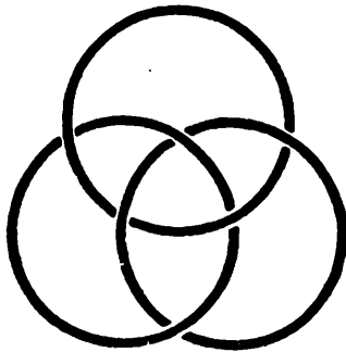
The Borromean knot 62
